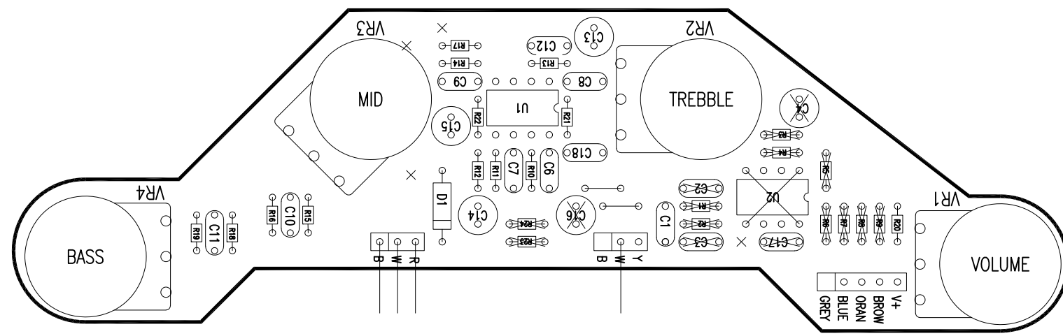
COMPONENT SIDE
